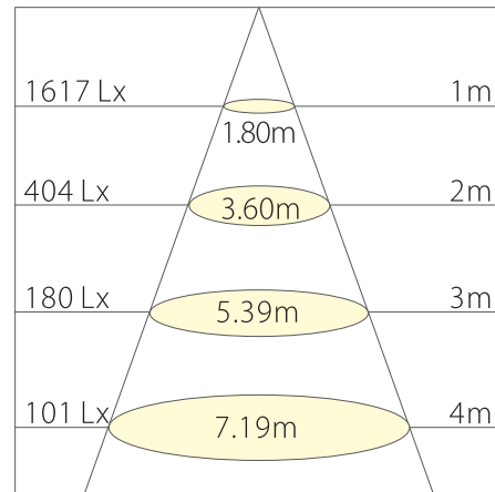
AAI Beam Diagram E(x) = Average lux
